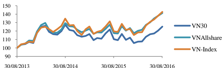
Indices performance from 30/08/2013 to 31/08/2016
