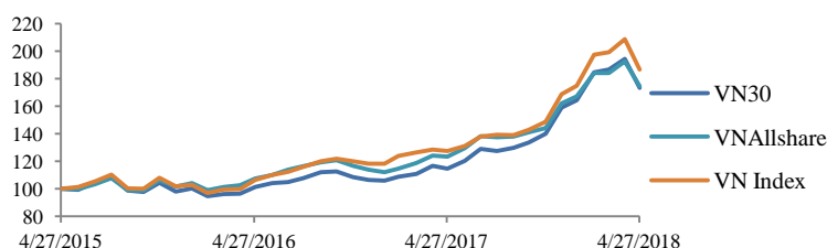
Indices performance from 27/04/2015 to 27/04/2018
