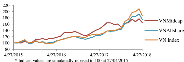
Indices performance from 27/04/2015 to 27/04/2018
