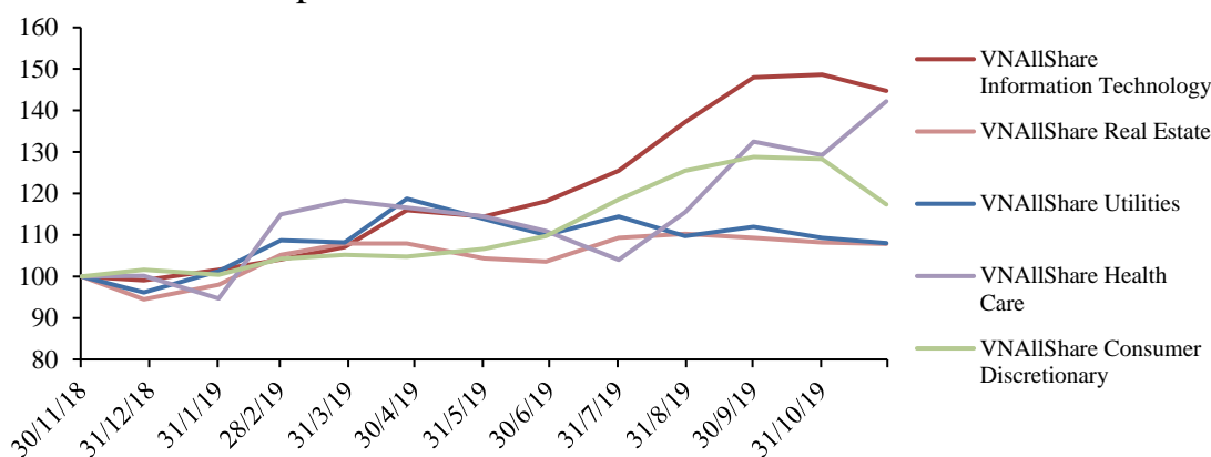
Indices performance from 30/11/2018 to 29/11/2019
