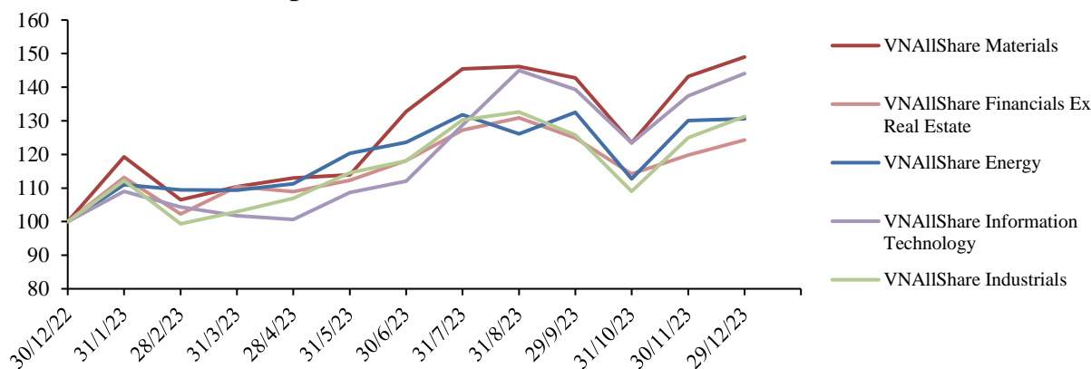
Indices performance from 30/12/2022 to 29/12/2023
